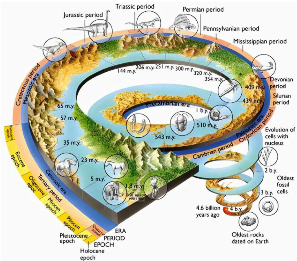
Visual and simplified depiction of the geologic time scale. Adapted from Press & Siever, 2000. Understanding Earth.
