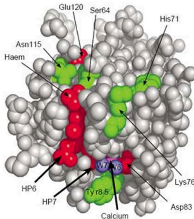
Figure 7. Surface view (space-filling) of cytochrome c_L . The outer haem propionate (HP6) is clearly exposed to solvent, as are the two water molecules (Wat6 and Wat7). Wat7 is bonded to the inner haem propionate (HP7). Asp83, one of the ligands to the calcium ion, has been proposed to be involved in interaction with methanol dehydrogenase together with Glu120, with the outer haem propionate (HP6) and with those residues coloured green. 24
