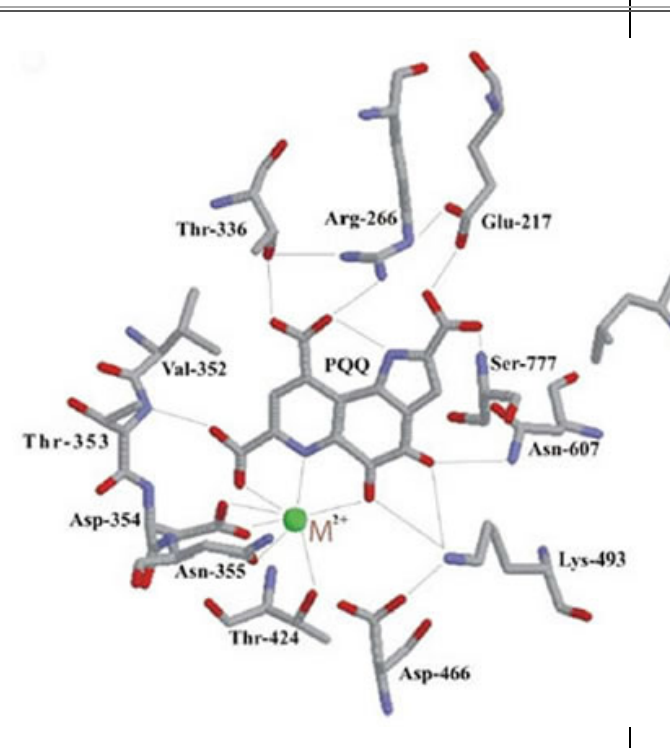
The active site of GDH [1]. The Metal may be Mg or Ca [3]
