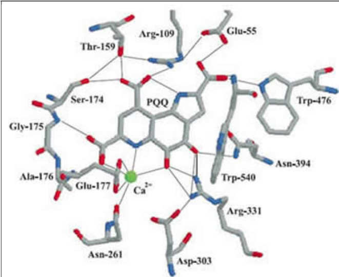
Fig. 2. The equatorial interactions of PQQ and the coordination of \text{Ca}^{2+} in the active site of MDH [10]. The figure also shows the proposed active site base (Asp 303 ) and Arg 331 which may also be involved in the mechanism.
