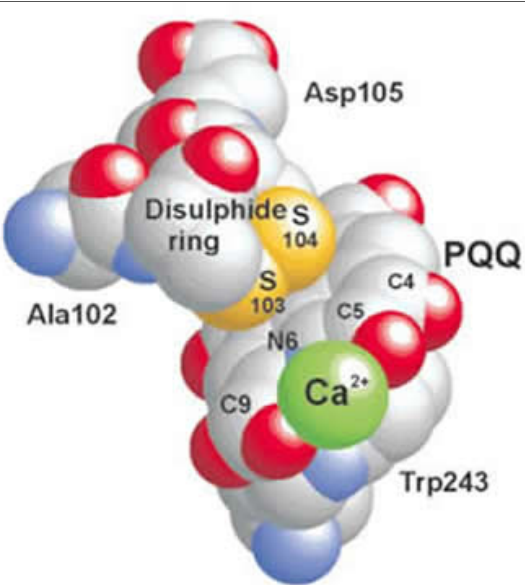
FIGURE 1: Disulfide bridge, PQQ, and \text{Ca}^{2+} in the active site of MDH.
