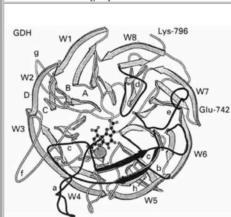
The 'propeller' structure of the model GDH [1]
